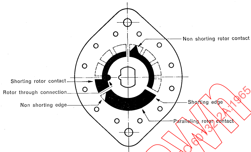
FIG. 4. — Indication of rotor blades.
