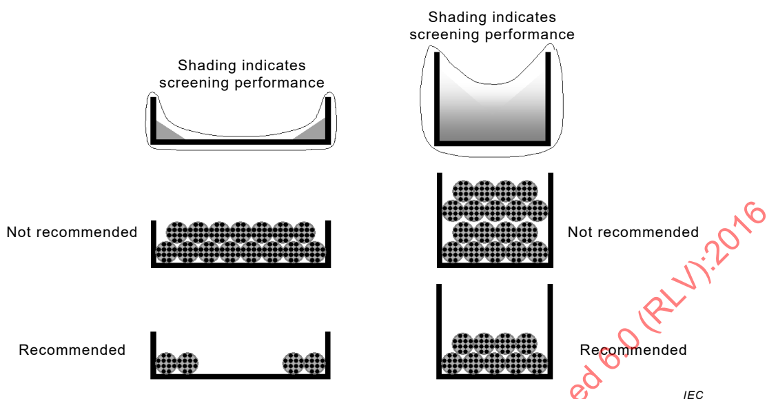
Figure H.4 – Cable arrangements in metal cable trays
