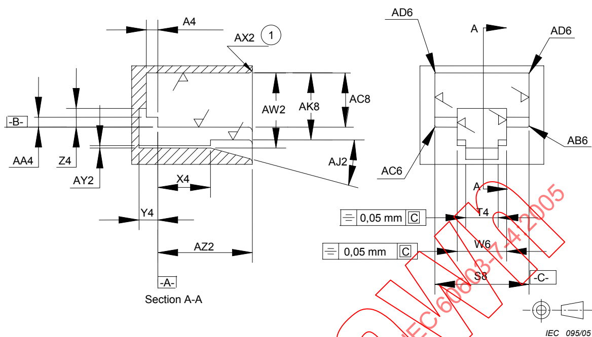
1 All around Figure 8 – Go gauge
