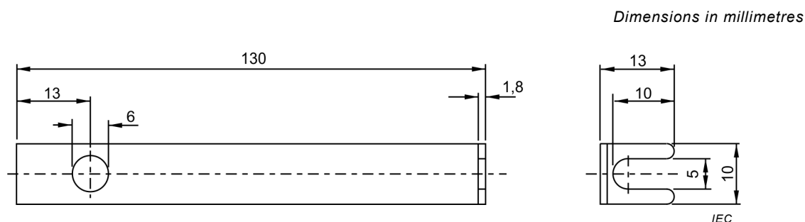
Figure 4 – Test strap
