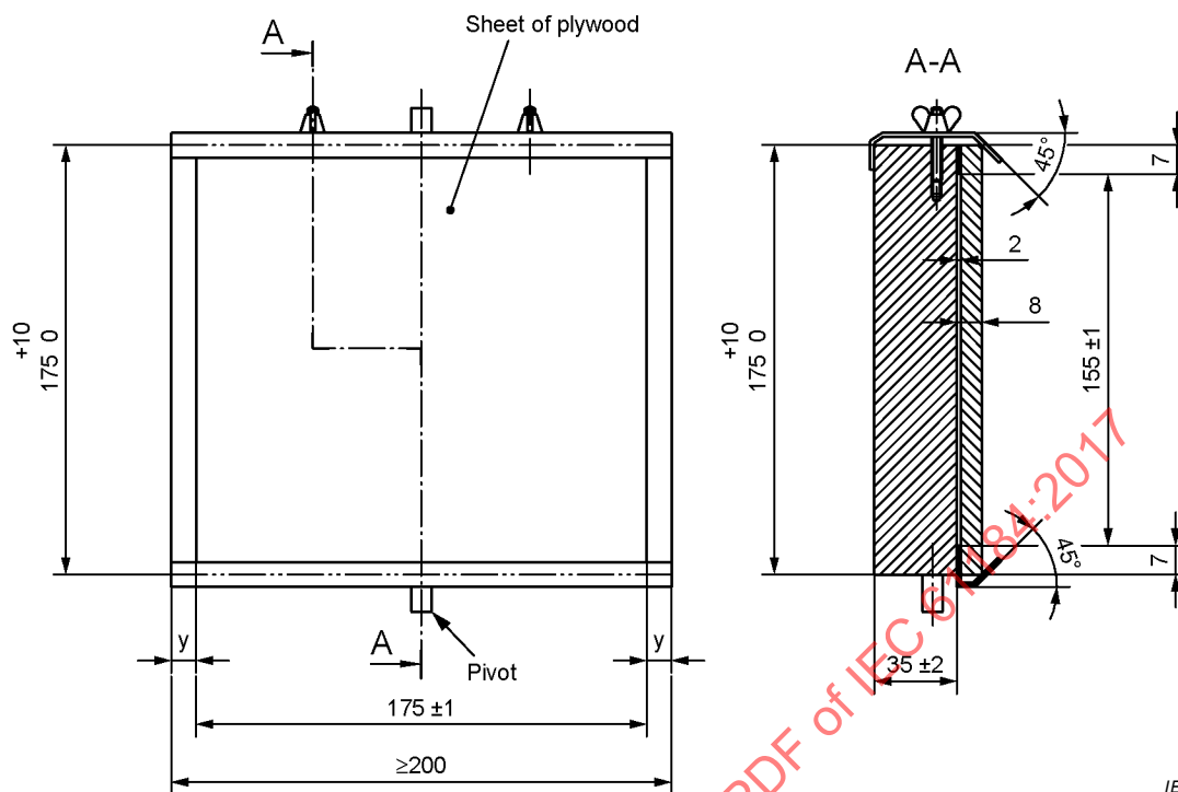
Figure 16 – Mounting support
