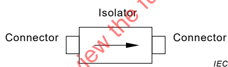
Figure 3 – Configuration C – Device containing connectors as an integral part of the device housing
