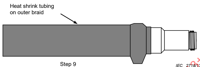
Figure C.3 – Symmetrical cables: preparation of cable end “A” (2 of 2)
