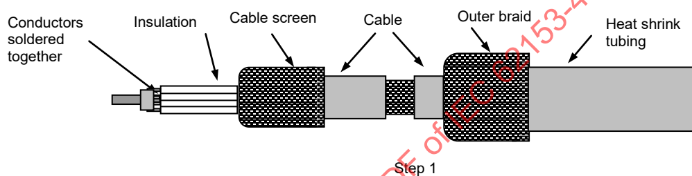
Figure C.3 – Symmetrical cables: preparation of cable end “A” (2 of 2)
