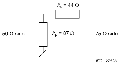
Figure B.3 – Coaxial impedance matching adapters (50 Ω to 75 Ω)
