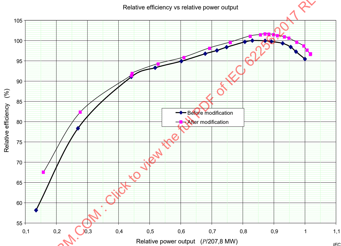
Figure 10 – Relative efficiency gain following modification of the blades on the La Grande 3 runner, in Quebec, Canada
