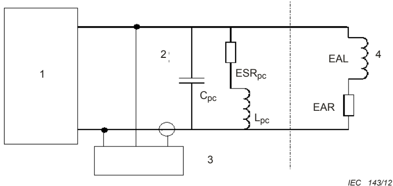
Figure D.1b – Internally a-type coupled plasma
