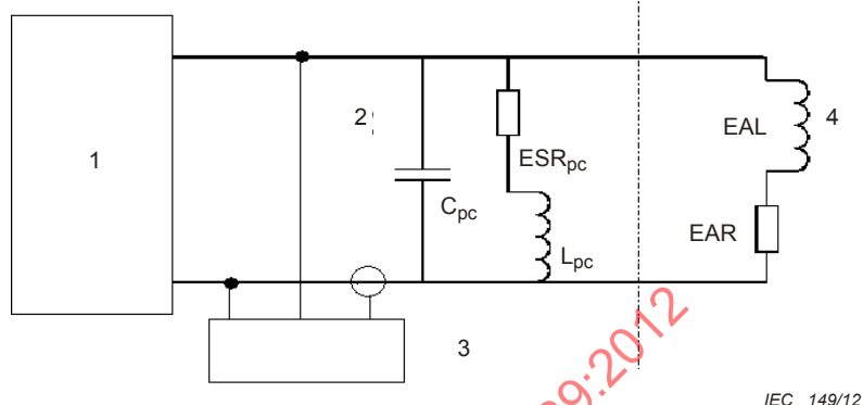
Figure D.3b – Internally a-type coupled plasma
