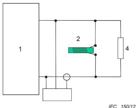
Figure D.3c – Internally b-type coupled plasma
