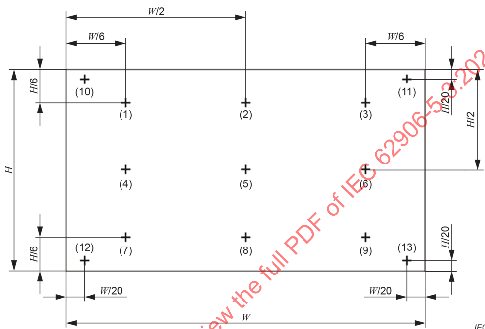
Figure 5 – Measurement points
