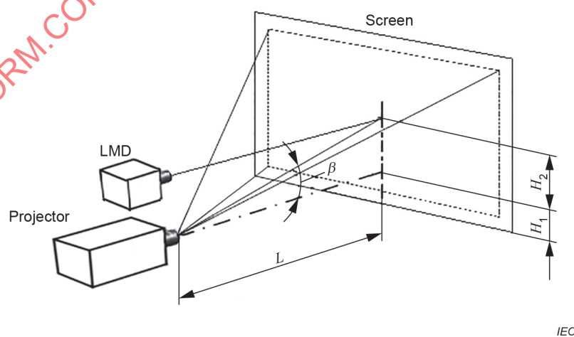
Figure 2 – Example of DUT setup
