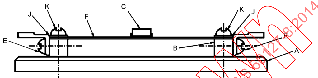
Figure 3b – Surface mount fuse resistor with particular overcurrent protection (printed circuit track on top)
