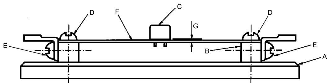
Figure 3a – Through-hole mount fuse resistor with particular overcurrent protection (printed circuit track underneath)
