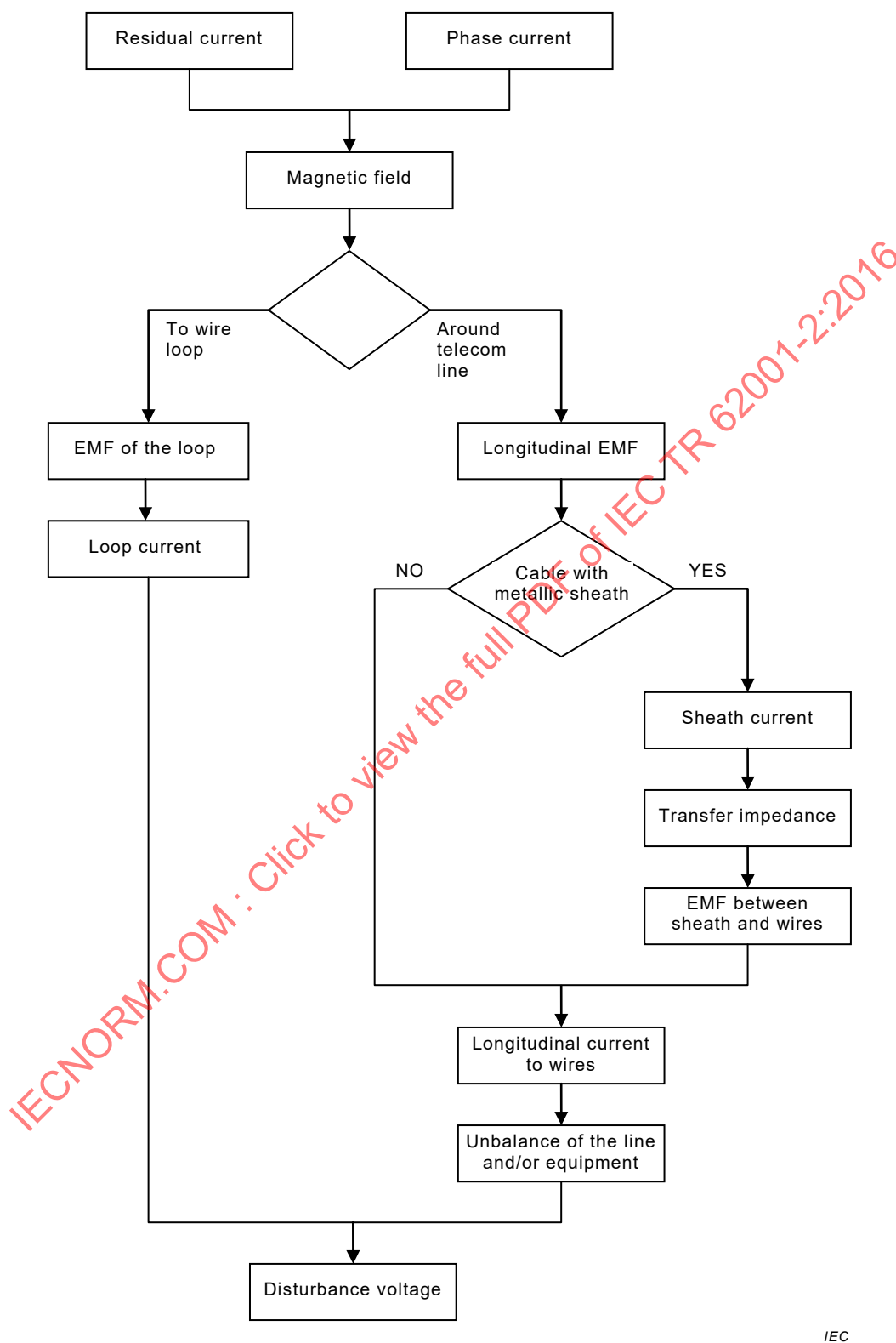
Figure A.3 – Flow-chart describing the basic telephone interference mechanism
