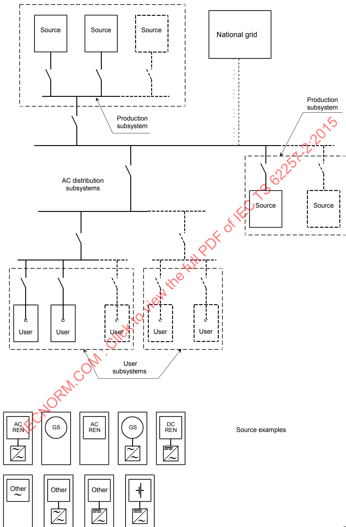
Figure 3 – General configuration of an electrification system
