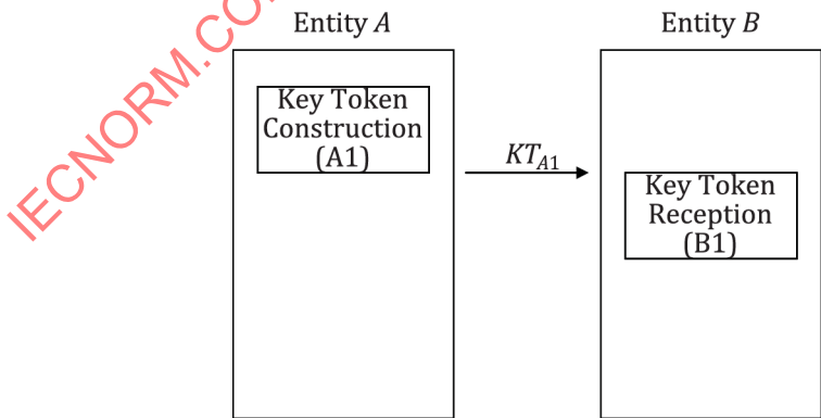
Figure 19 — Public key transport mechanism 1
