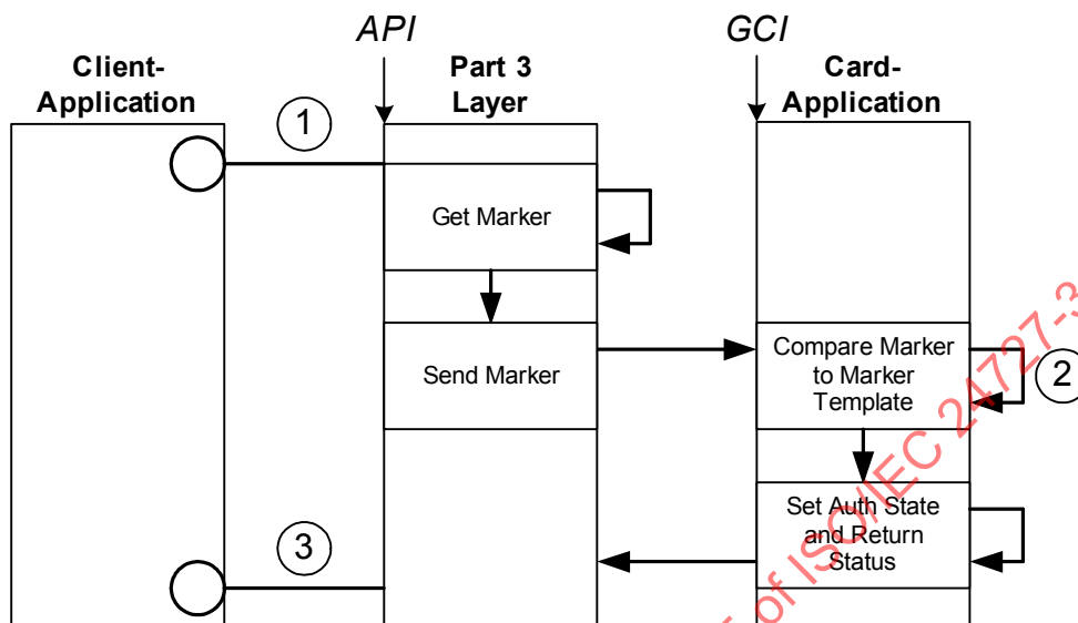
Figure A.8 — Biometric Compare
