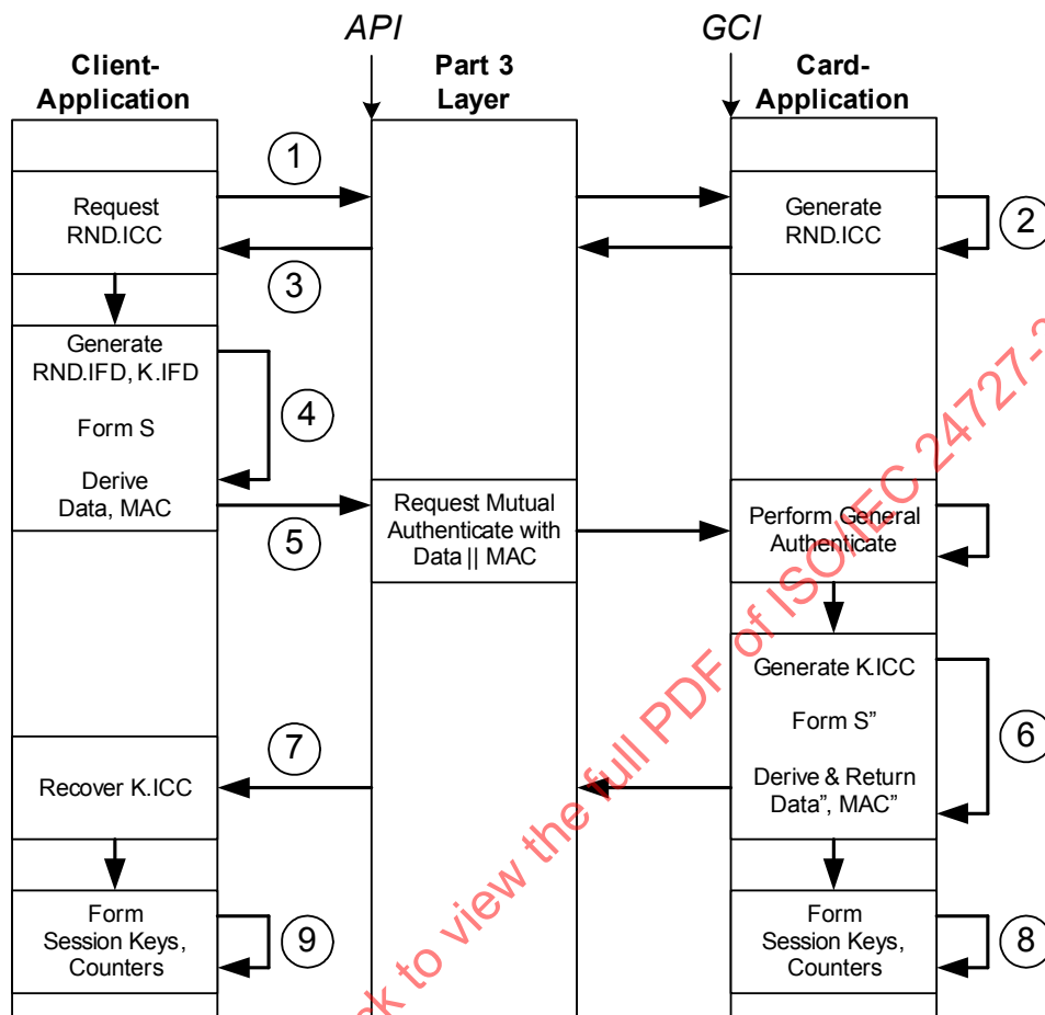
Figure A.10 — Client-Application Mutual Authentication with Key Establishment
