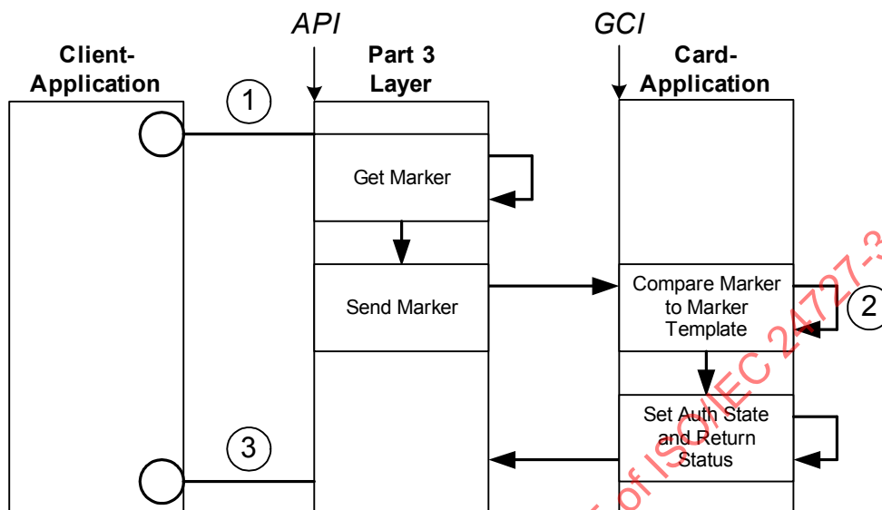
Figure A.6 — Compare
