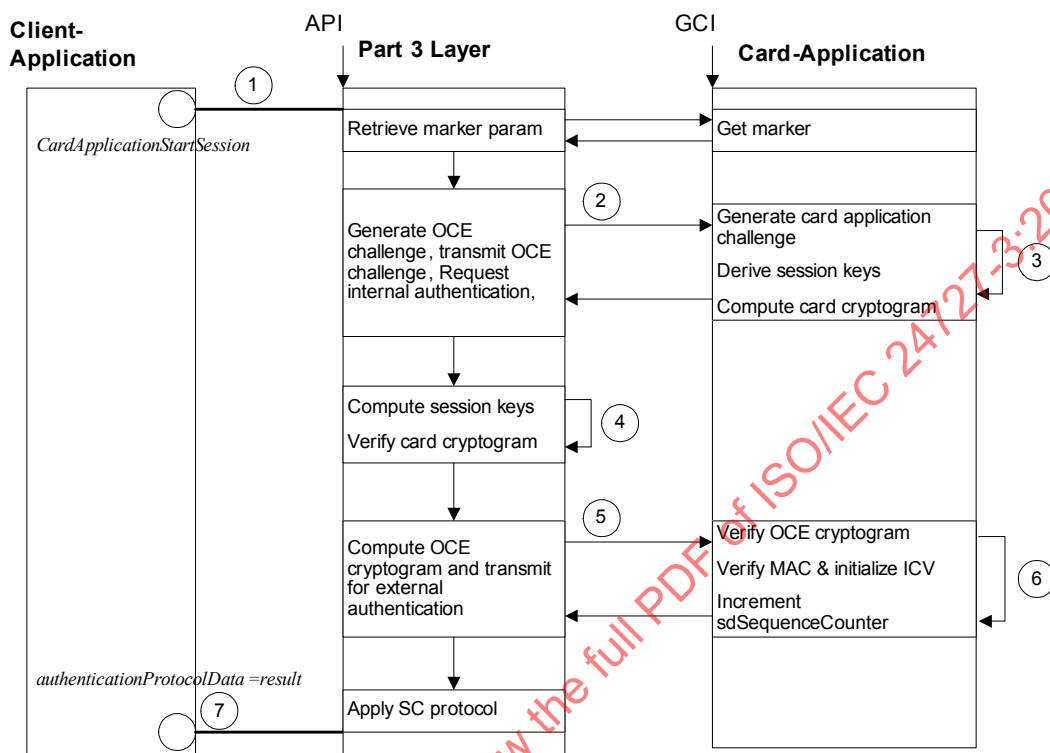
Figure A.21 — GP Symmetric Authentication (Explicit Mode)
