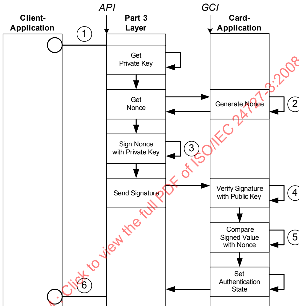
Figure A.3 — Asymmetric External Authenticate
