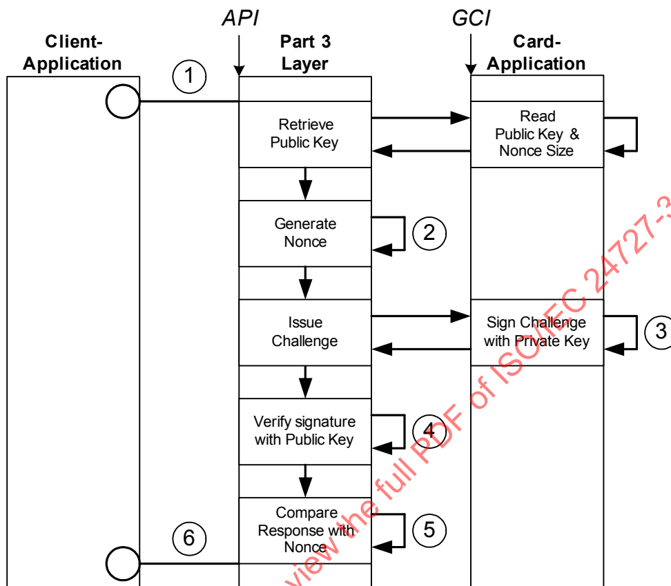
Figure A.2 — Asymmetric Internal Authenticate
