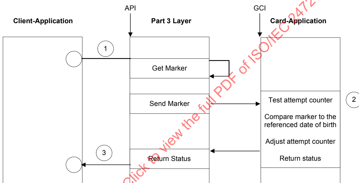
Figure A.14 — Age Attainment
