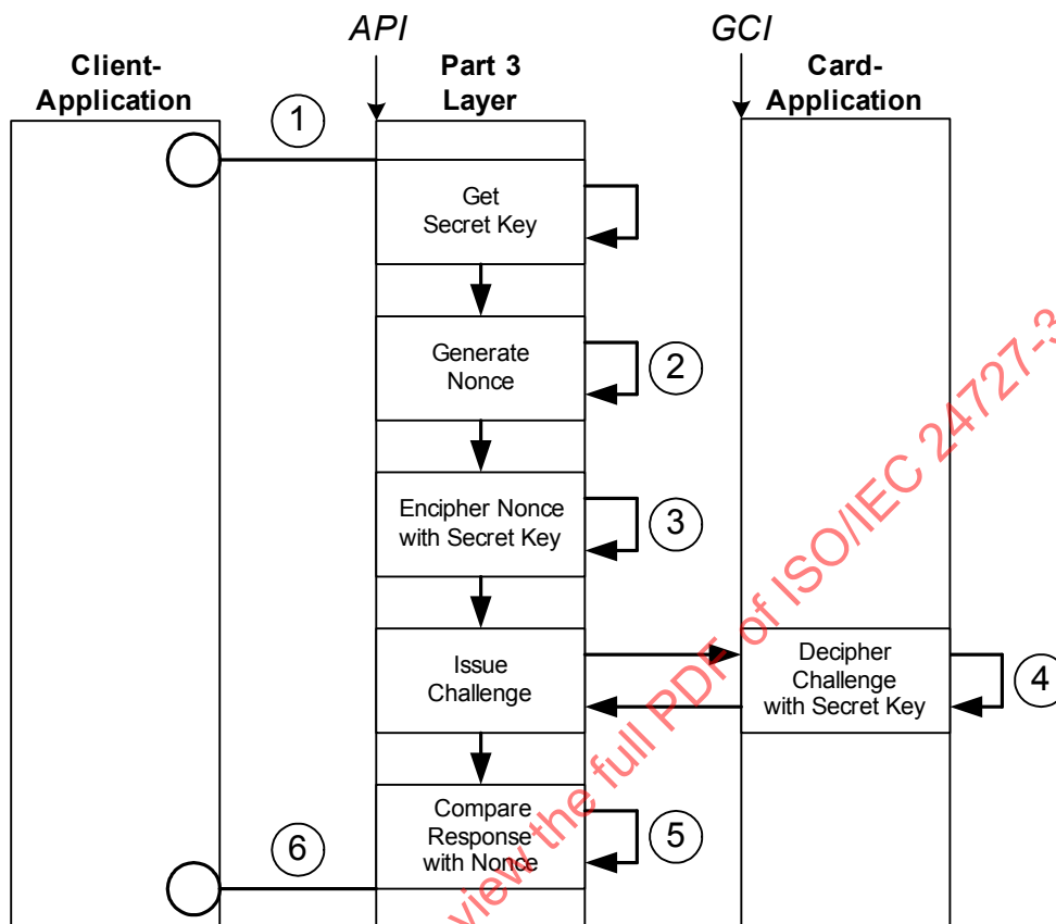
Figure A.4 — Symmetric Internal Authenticate
