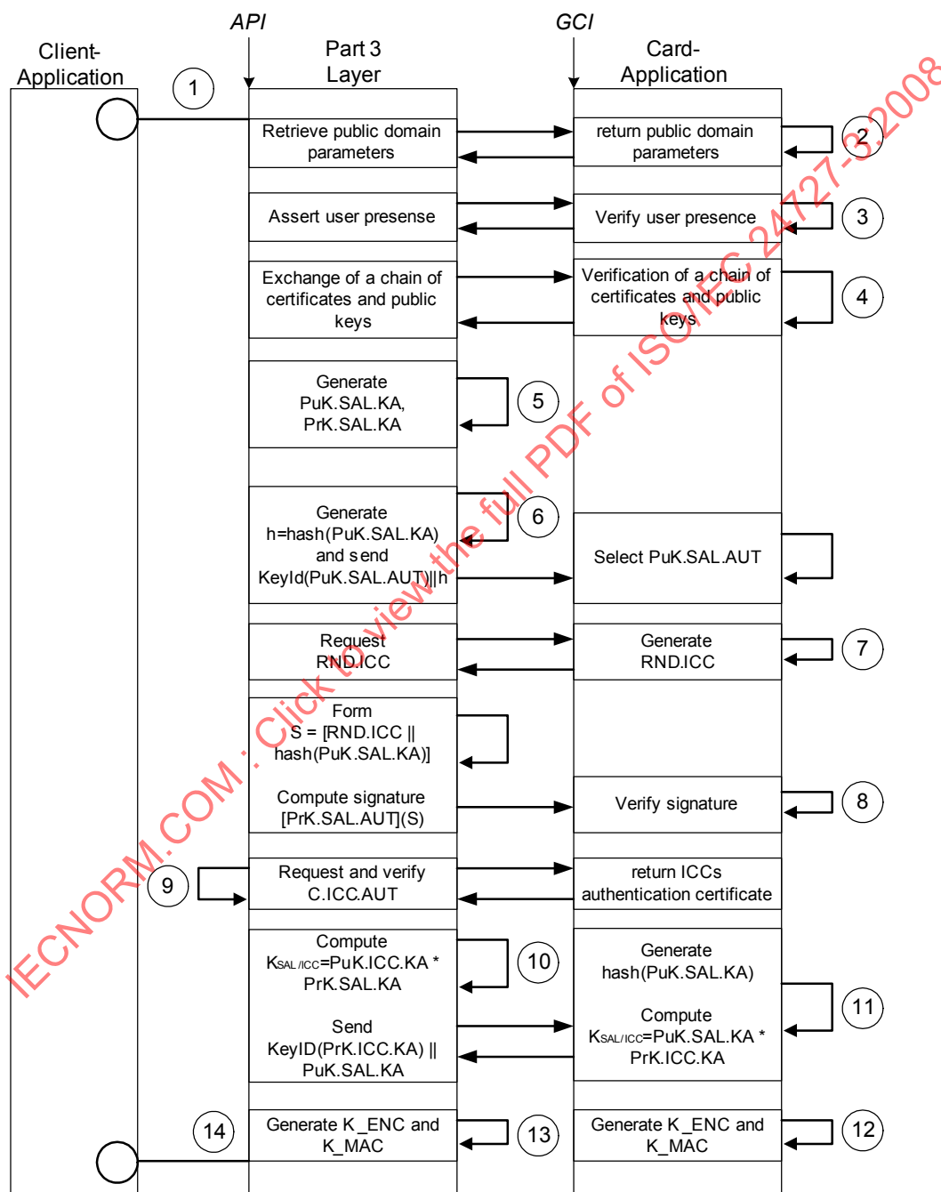
Figure A.13 — Key Transport with mutual authentication based on RSA
