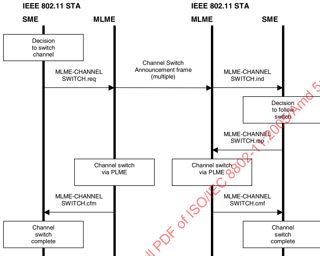
Figure 67e—Channel switch
