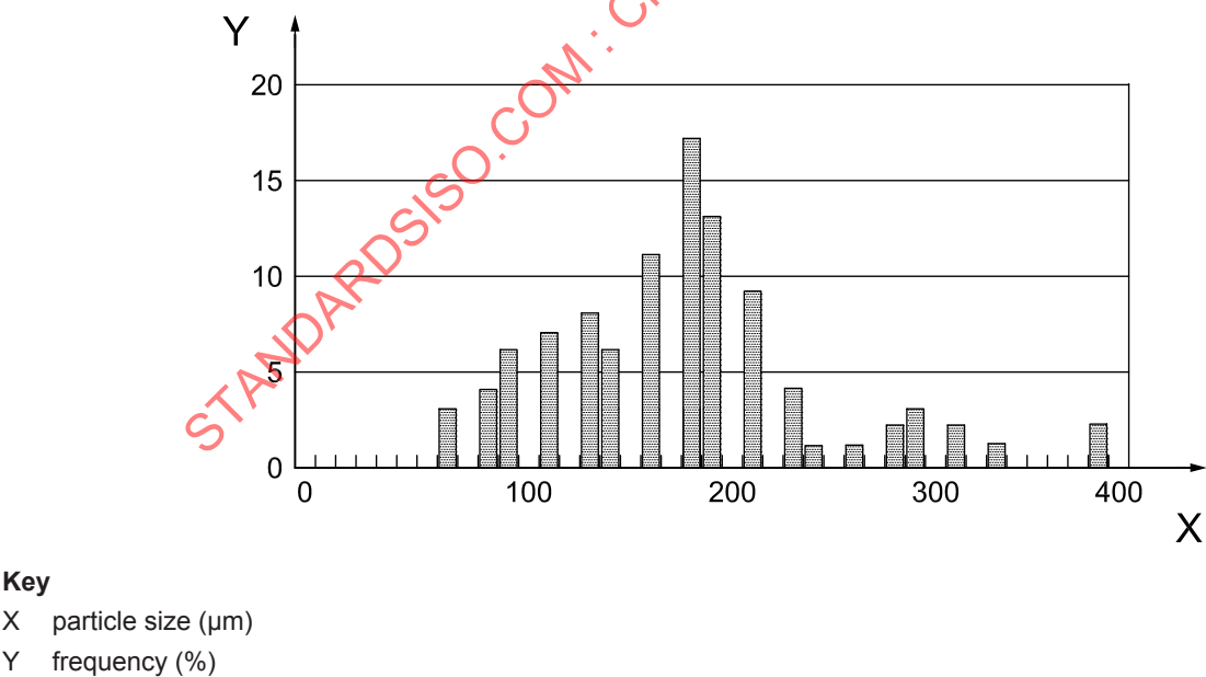
Figure A.2 — Particle size distribution of PCL powder milled using a mixer and then sieved
