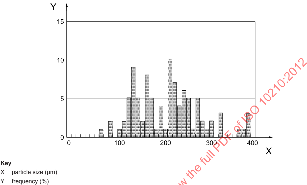
Figure A.1 — Particle size distribution of PLA powder milled using a mixer and then sieved
