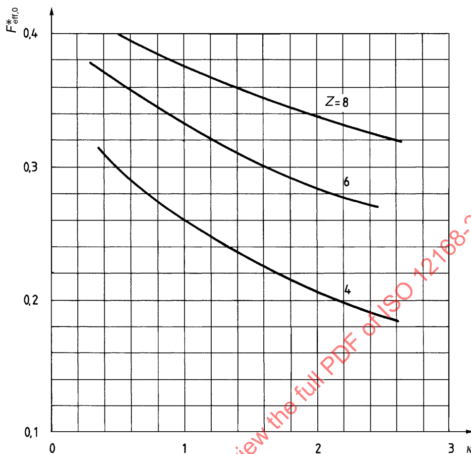
Figure 3 — Characteristic values of load-carrying capacity F_{\text{eff},0}^* for a relative eccentricity \varepsilon = 0,4 as a function of the resistance ratio \kappa and for different numbers of recesses Z , \alpha = 0 ; \omega = 0 ; \xi = 1
