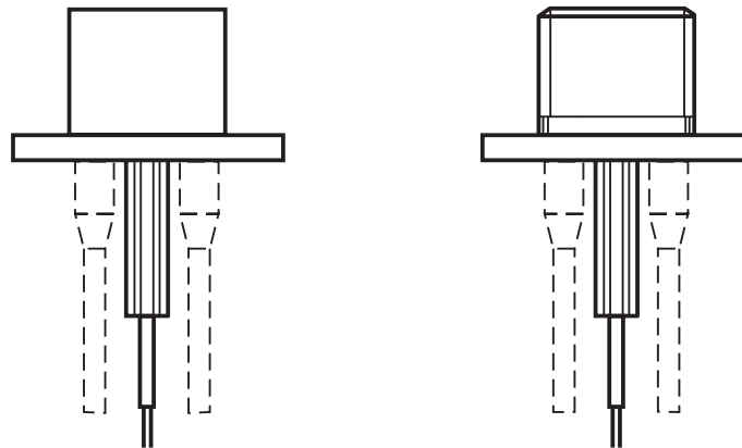
Figure 6 — Flanged heat flux meter (left) and flanged and threaded heat flux meter (right)
