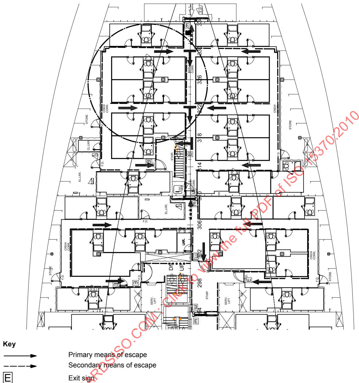
Figure G.5 — Example relating to 6.2.1 of a typical arrangement of LLL avoiding circulation around the same accommodation space
