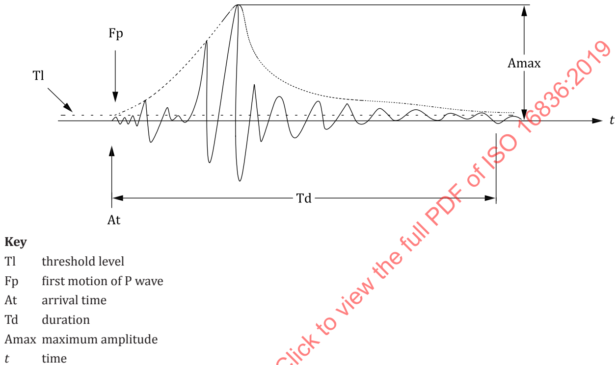
Figure 5 — AE waveform parameters
