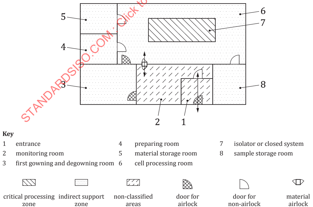
Figure C.7 — Example of material flow in a containment facility with isolator
