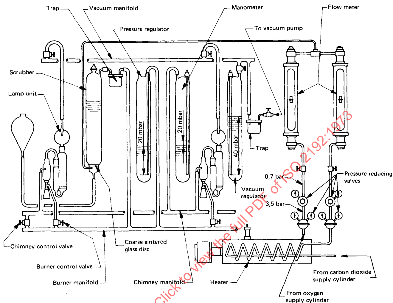
FIGURE 2 – Schematic diagram of carbon dioxide-oxygen supply manifold and lamp system
