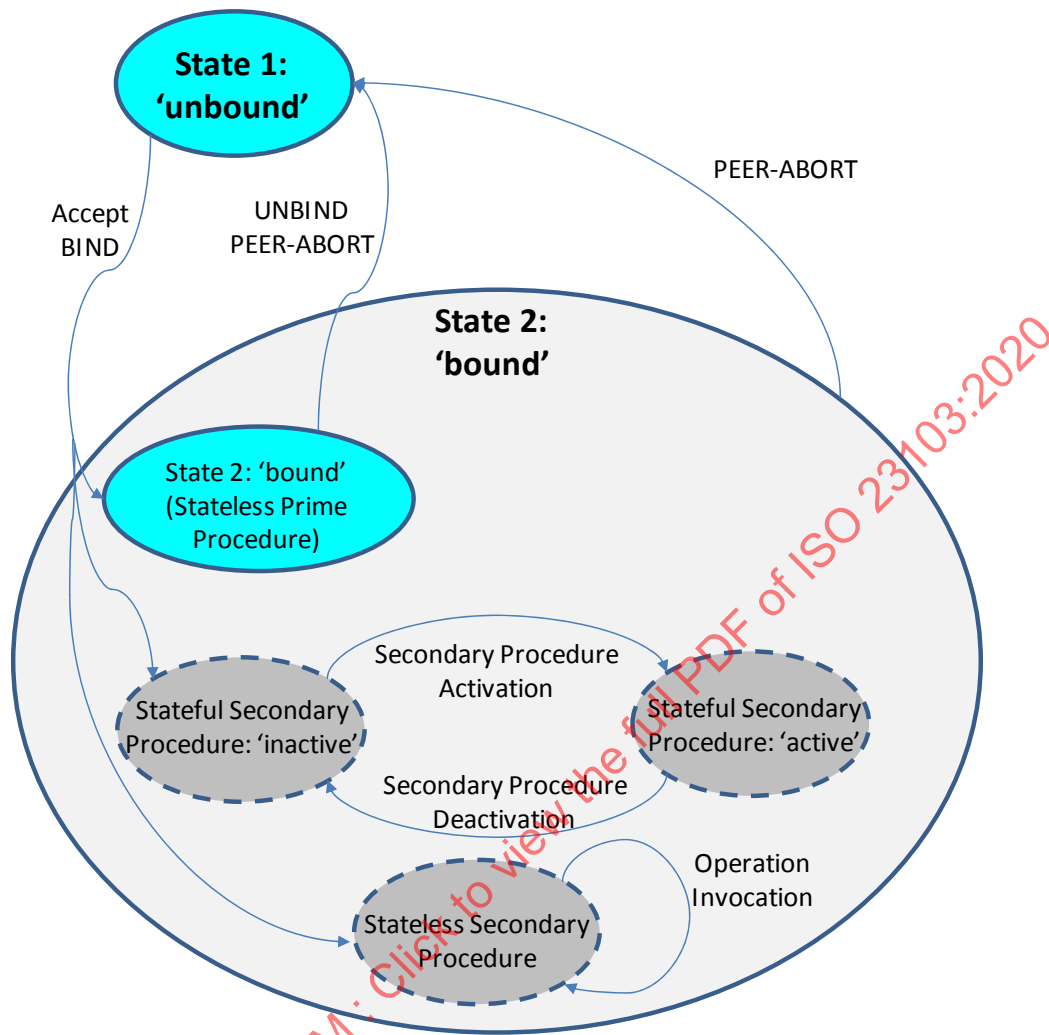
Figure 2-3: Service and Procedure States (Stateless Prime Procedure)
