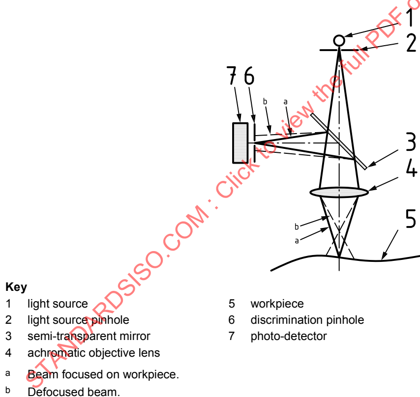
Figure B.1 — Principle of a confocal sensor
