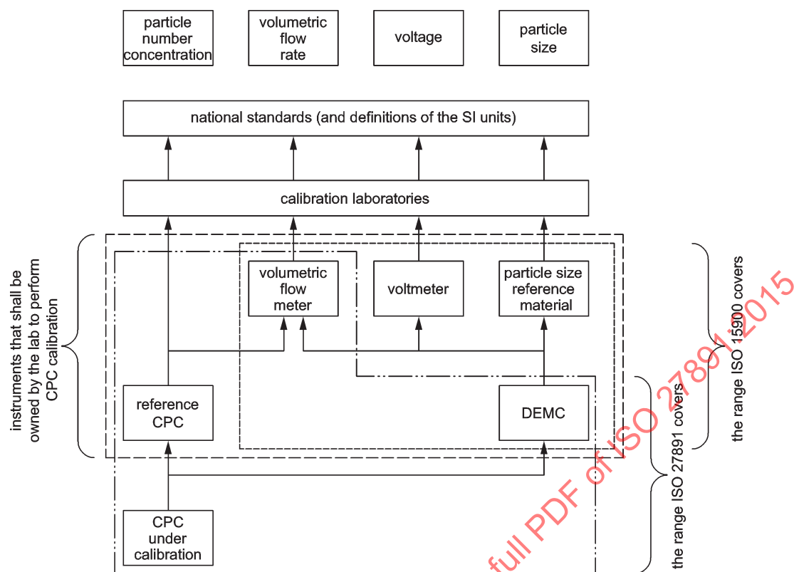
Figure E.2 — Traceability diagram for calibration with a reference CPC
