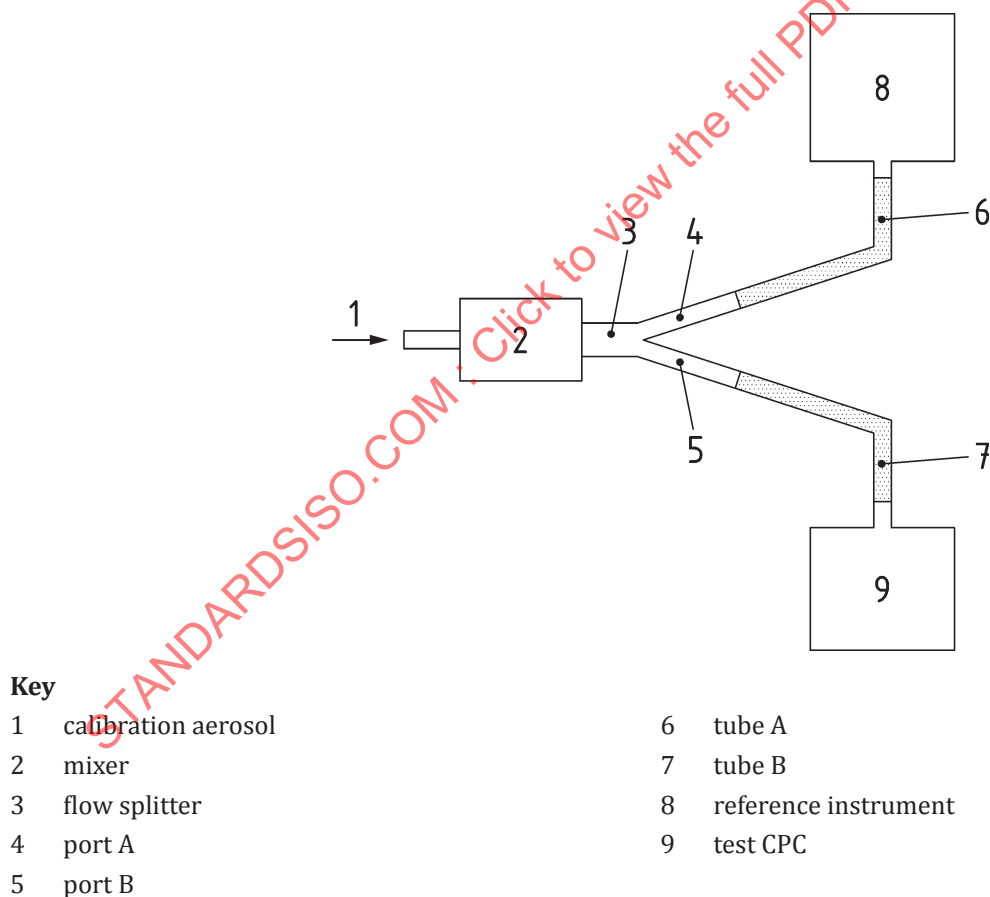
Figure G.1 — First connection configuration of the flow splitter and the tubes after it
