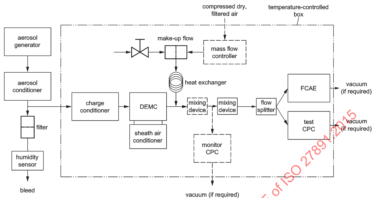
Figure 4 — Typical calibration setup with FCAE as reference instrument
