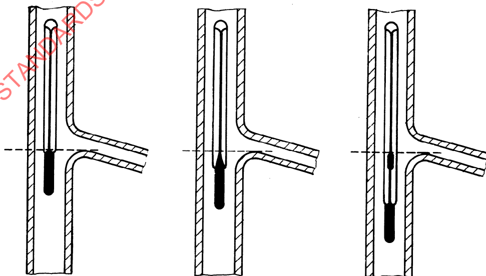
Figure 5 — Position of thermometer in distillation flask
