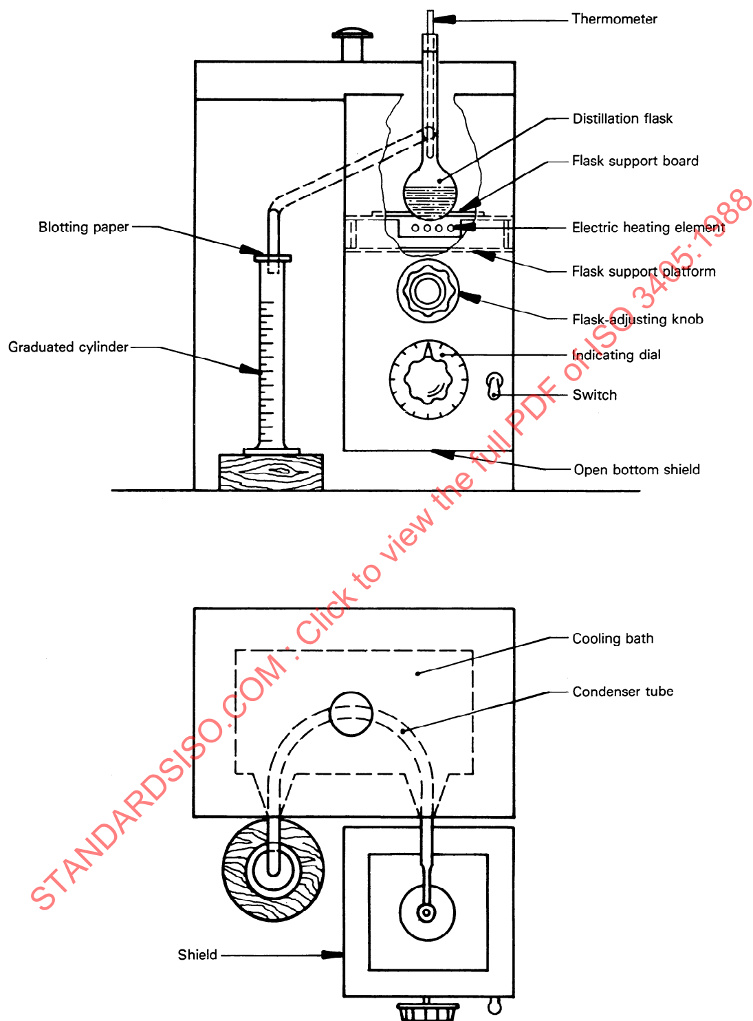
Figure 3 — Apparatus assembly using electric heater
