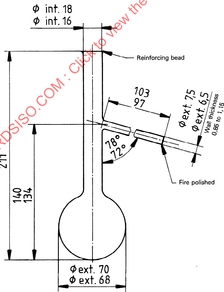
Figure 1 — Distillation flask
