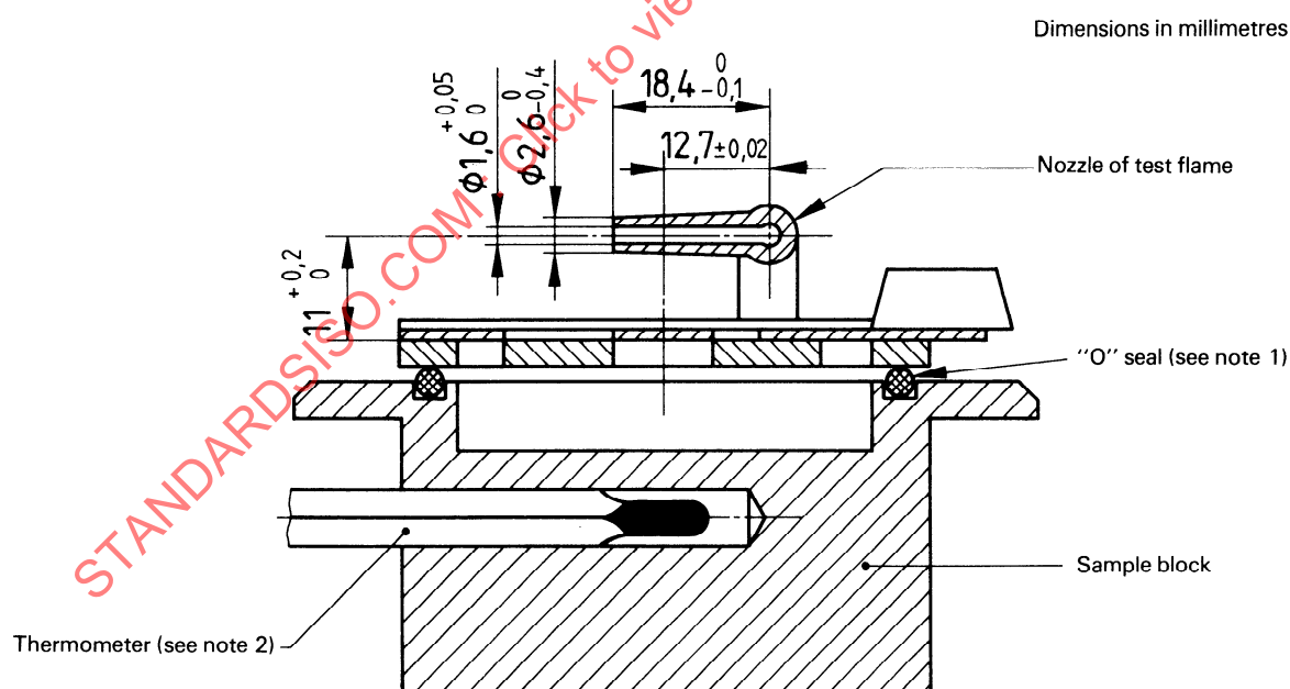
Figure 2 — Section of block through nozzle of test flame
