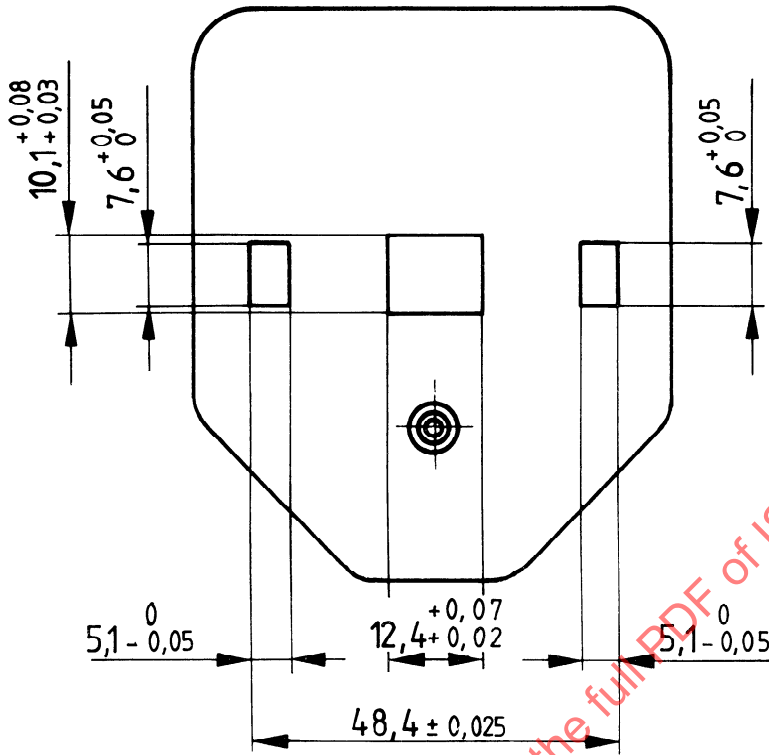
Figure 3 — Cover (brass or other suitable metal, approximately 2 mm thick)
