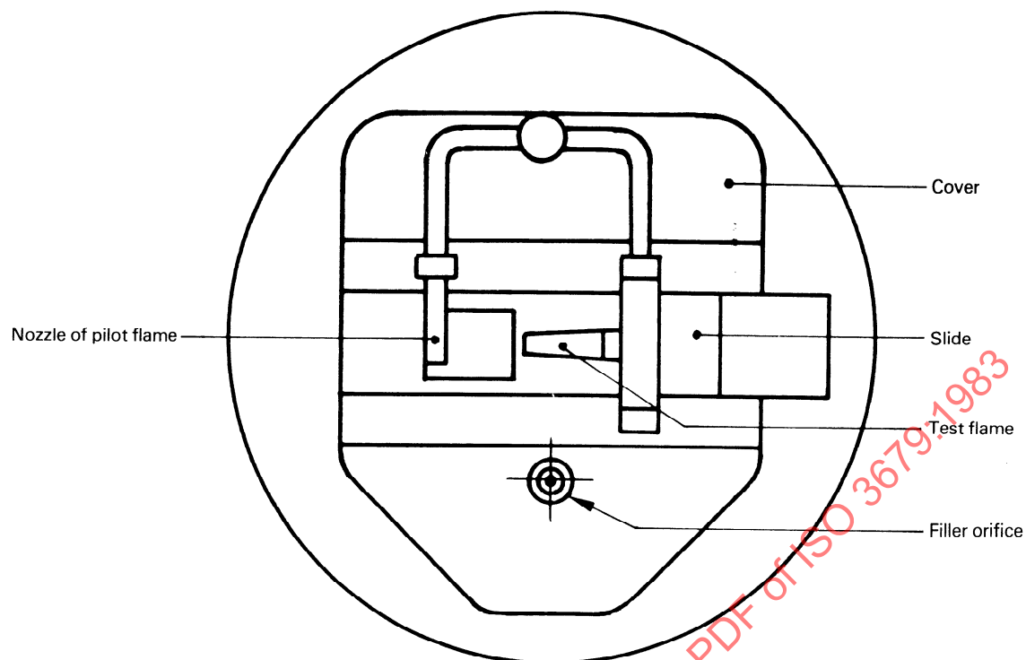
Figure 1 — Plan diagram of flashpoint tester
