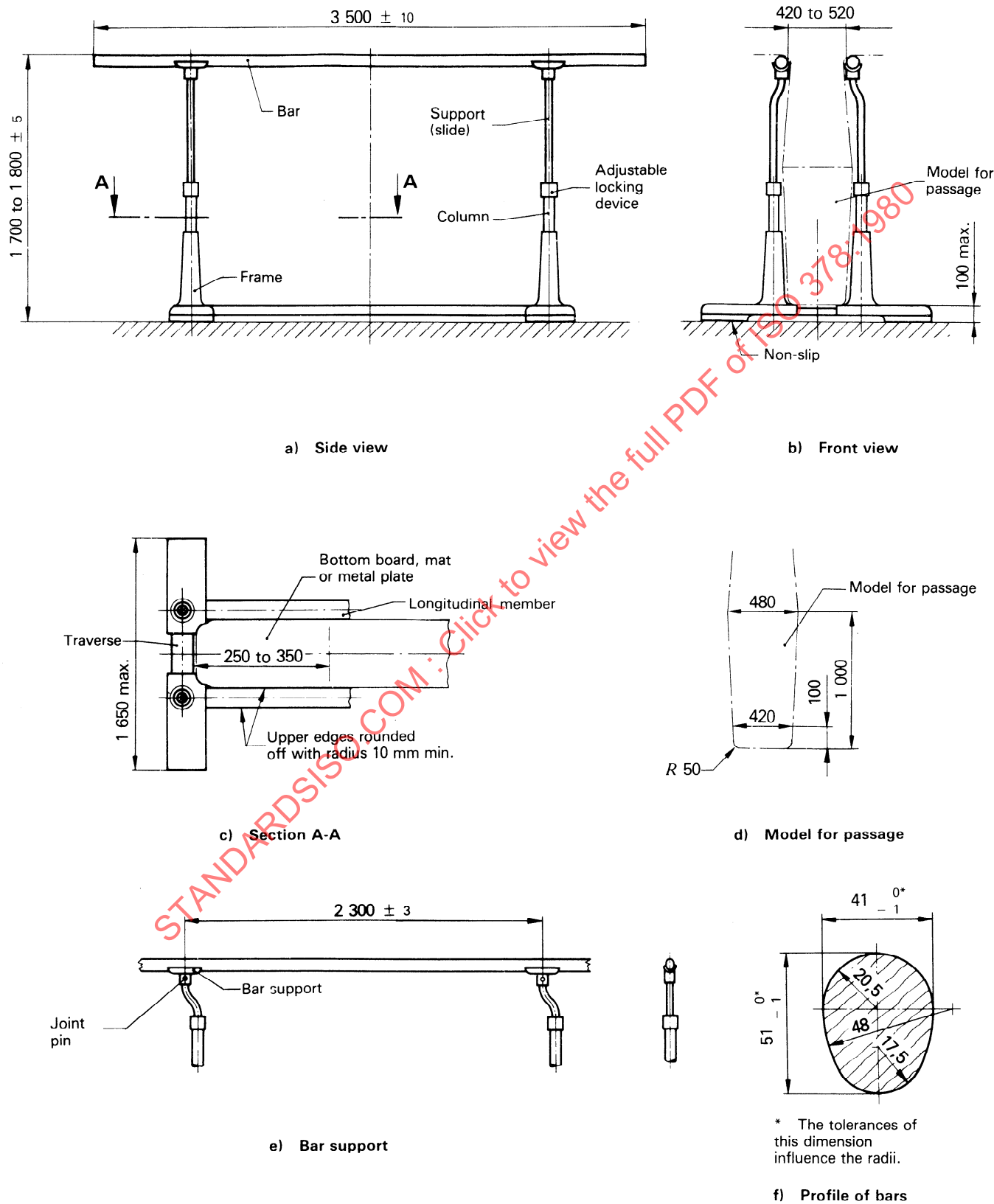
Figure 1 — Dimensions of parallel bars
