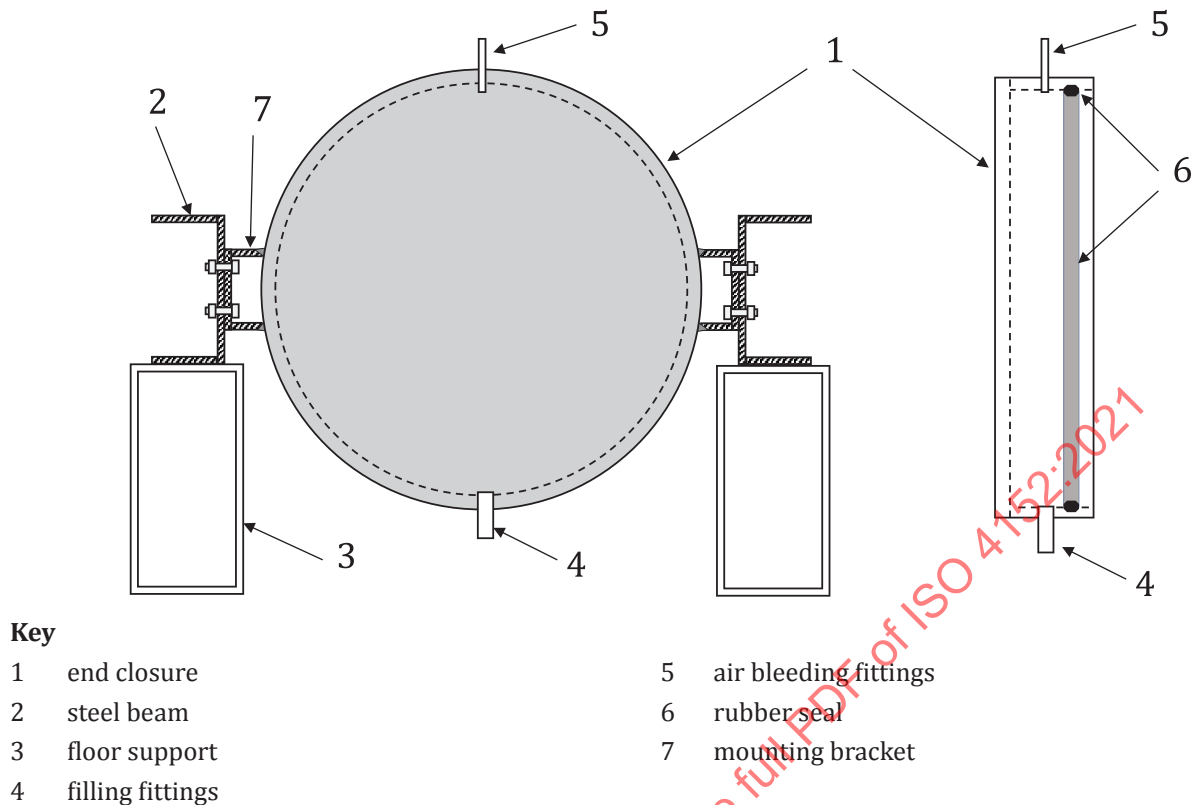
Figure 2 — Typical detail of end closure
