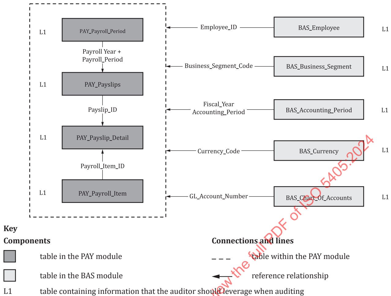
Figure 3 — Table relation diagram of the PAY module
