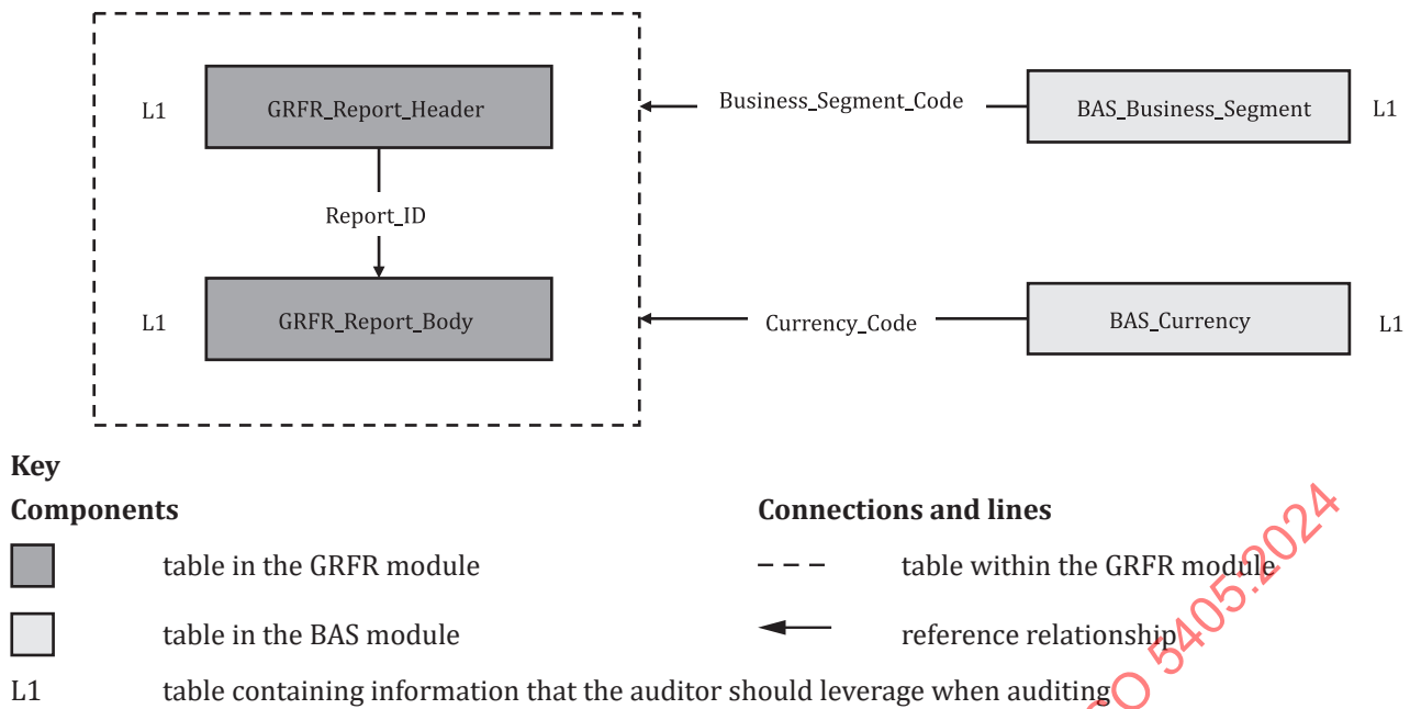
Figure 2 — Table relationship diagram of the GRFR module
