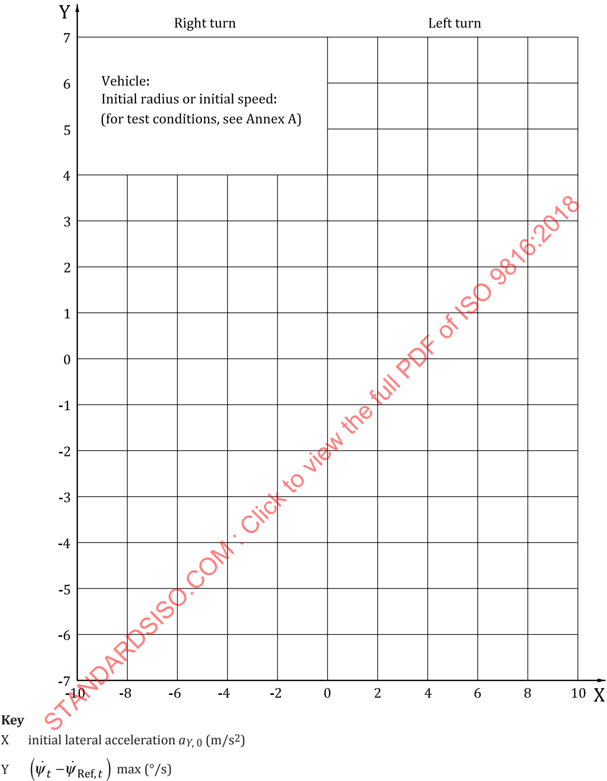
Figure B.6 — The maximum value of the difference between the yaw velocity during power-off \dot{\psi}_t and the affiliated reference yaw velocity \dot{\psi}_{\text{Ref},t} as a function of the initial lateral acceleration a_{Y,0}
