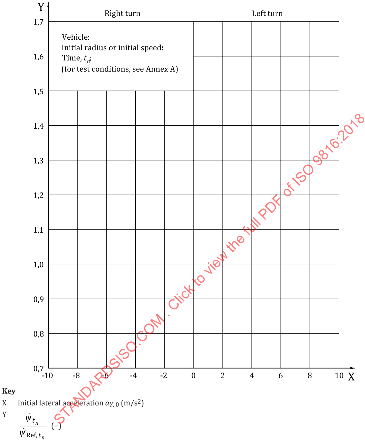
Figure B.3 — The ratio of the value of the yaw velocity at time t_n to the value of the reference yaw velocity at time t_n as a function of the initial lateral acceleration a_{Y,0}
