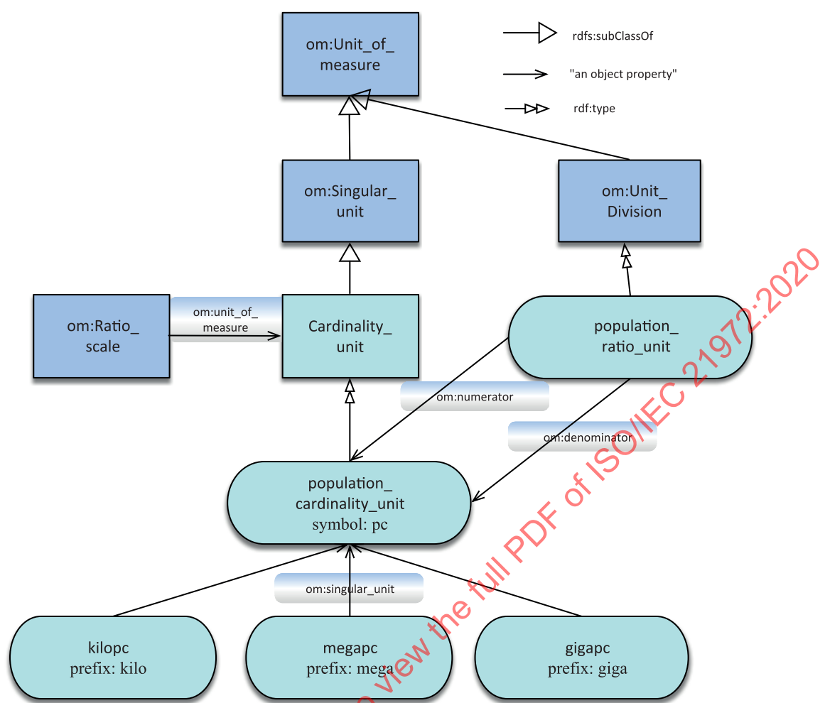
Figure 10 — Population_ratio_unit definition (3 of 3)
