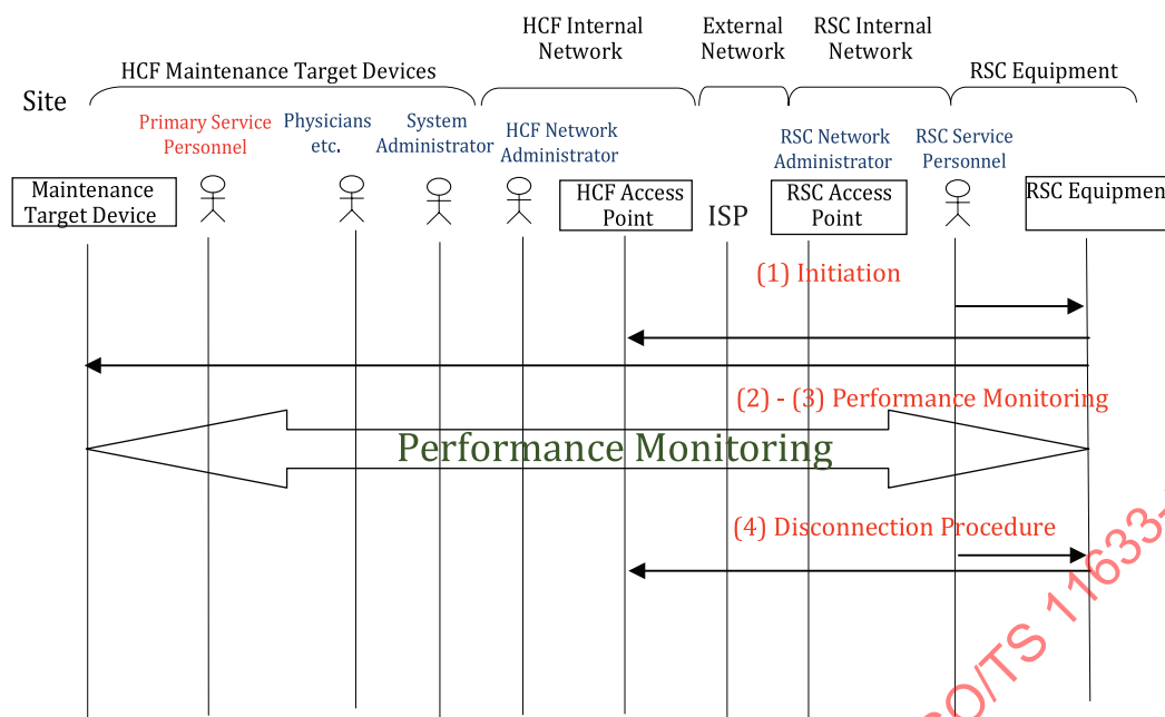
Figure A.4 — Workflow in the case of performance monitoring
