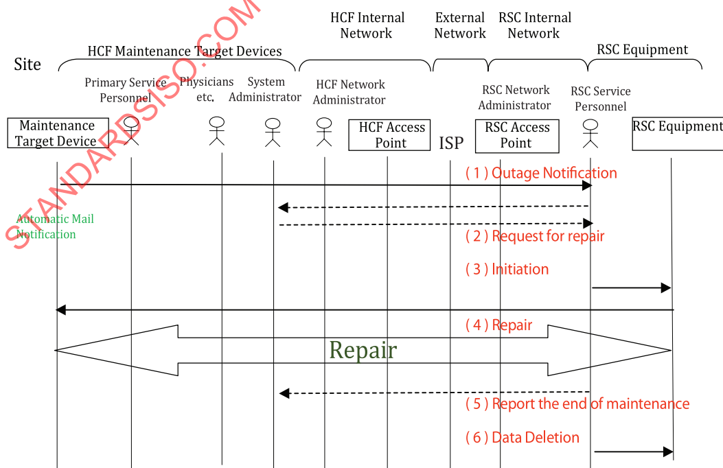
Figure A.1 — Workflow in the case of trouble shooting outages
