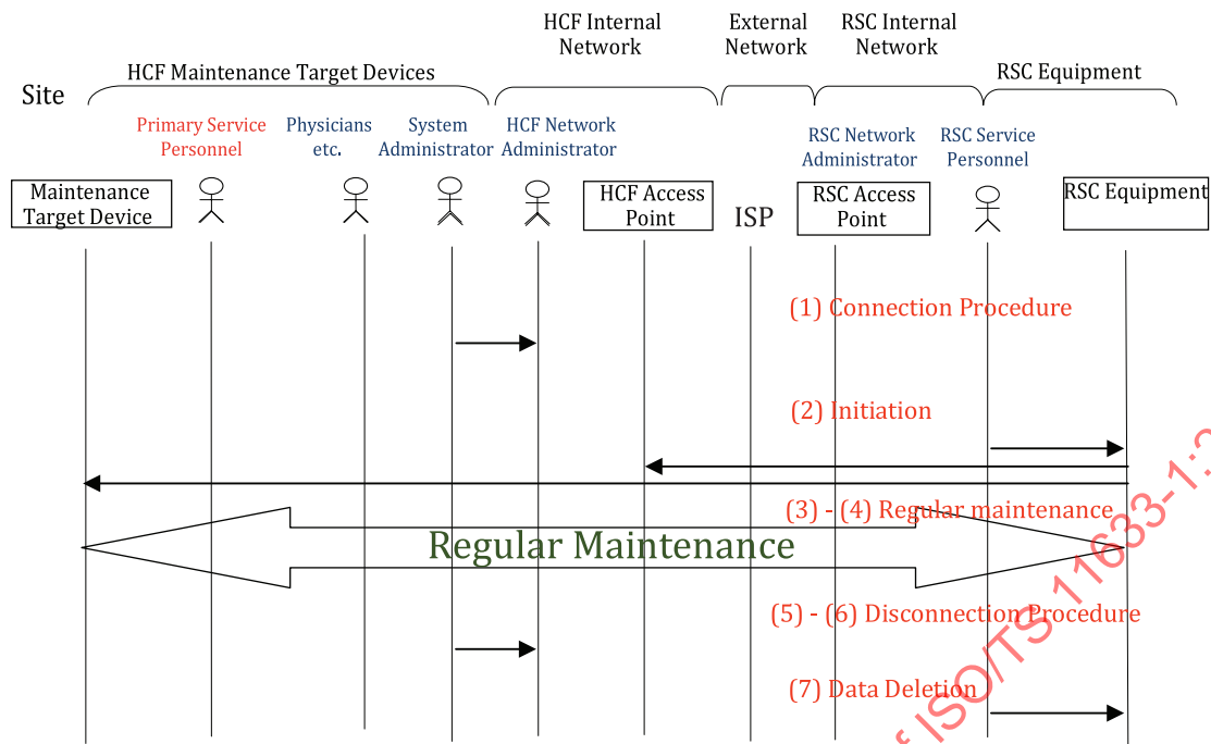
Figure A.2 — Workflow in the case of scheduled maintenance
