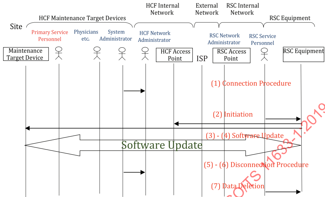
Figure A.3 — Workflow in the case of software updates
