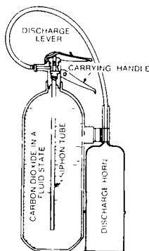
Figure D-4-3.1(a) Carbon Dioxide Extinguisher.
