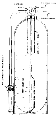
Figure D-4-2.1 Stored-Pressure AFFF Extinguisher.
