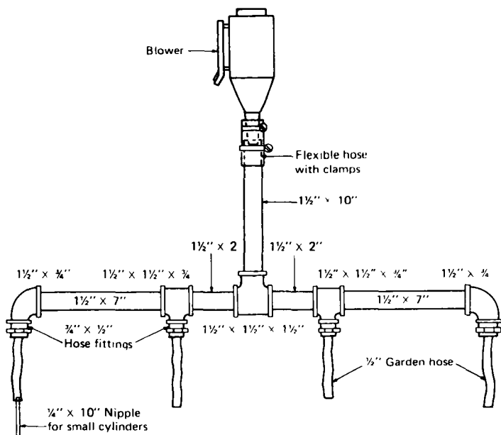
Figure A-5-5.3.2 Cylinder Drying Device.
