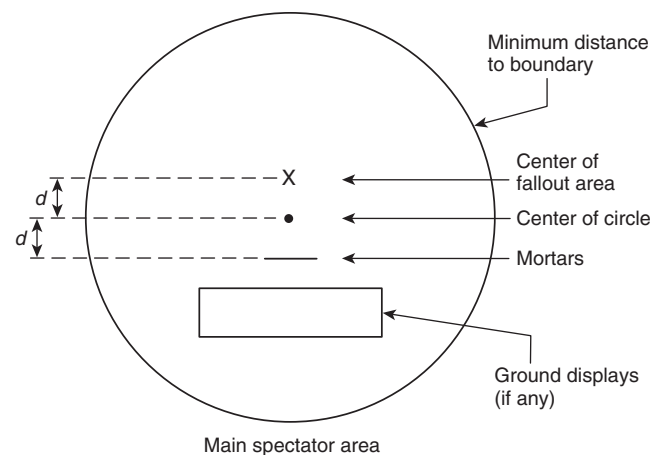
FIGURE A.5.2.1.3 Typical Layout for a Display Site Using Angled Mortars. The distance, d , should be at least one-sixth but not more than one-third the radius of the circle, indicating the minimum distance to the secured boundary.
