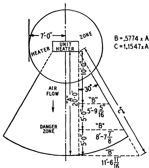
Fig. 3656(a). Heater and Danger Zones at Unit Heaters.
