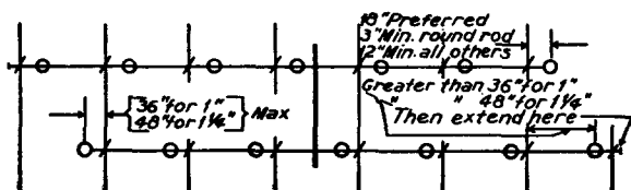
Fig. 3551. Distance Between Hangers When Using Steel Pipe (See also 3561 and 3564).
