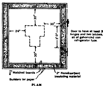
Fig. 5258-5. Dry-Pipe Valve Enclosure — Combustible Construction.
