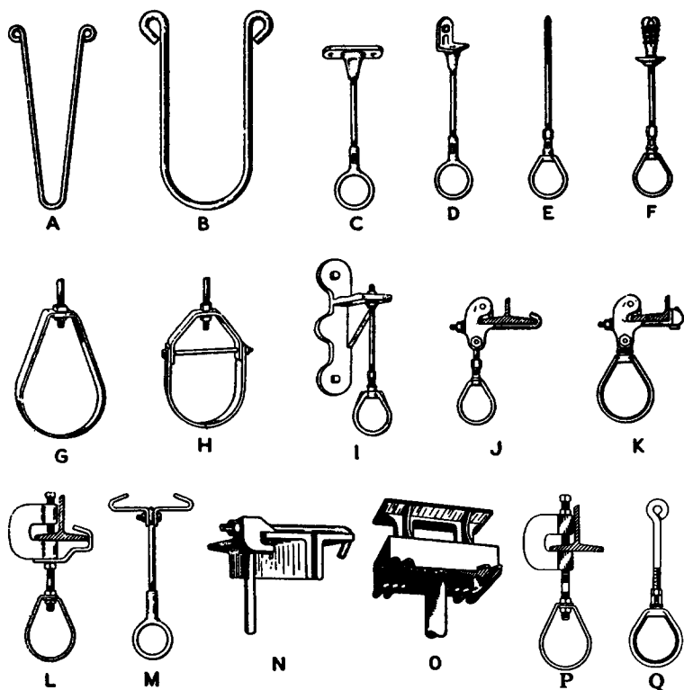
Fig. 3516. Common Types of Acceptable Hangers.
