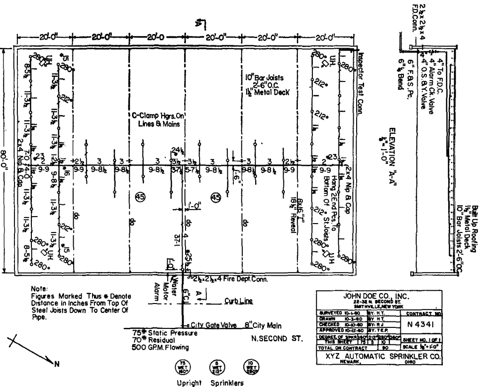
Fig. 1440-1. Typical Working Plans.
