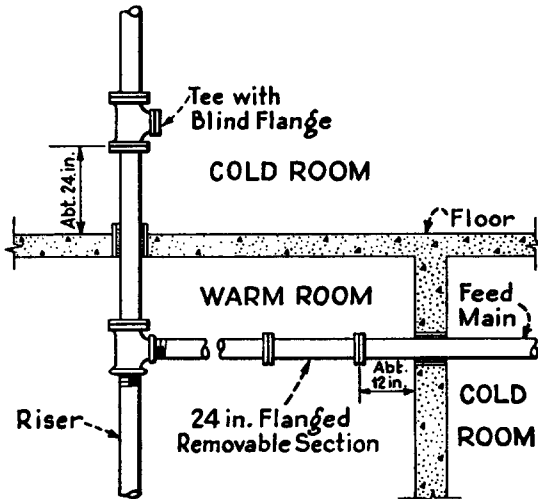
Fig. 5262-2. Fittings in Feed Main or Riser Passing Through Wall or Floor from Warm Room to Cold Room.
