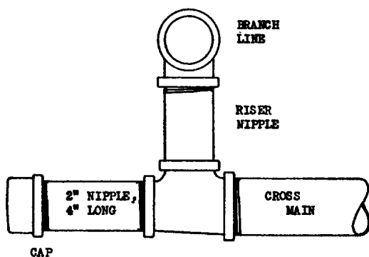
Fig. 3063. Flushing Connection.
