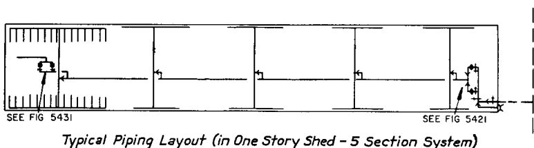
Fig. 5411. Typical Piping Layout for Combined Dry-Pipe and Pre-Action Sprinkler System.
