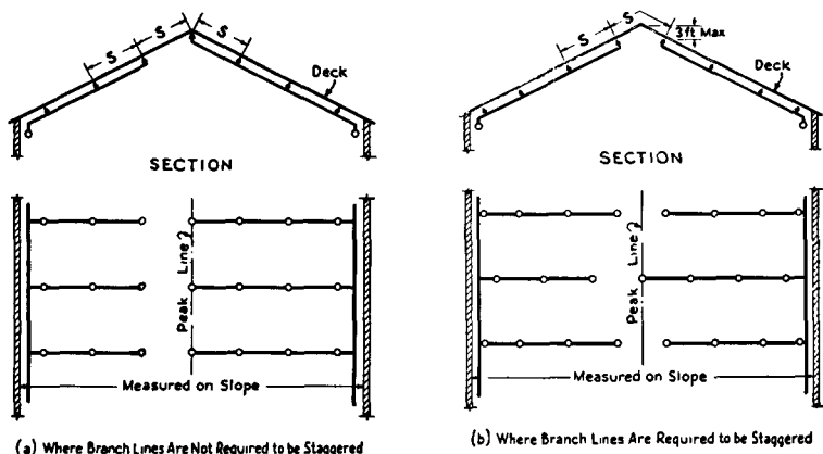
Fig. 4306(a). Sprinklers at Pitched Roofs. Branch Lines Run Up the Slope.
