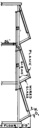
SECTION B-B
