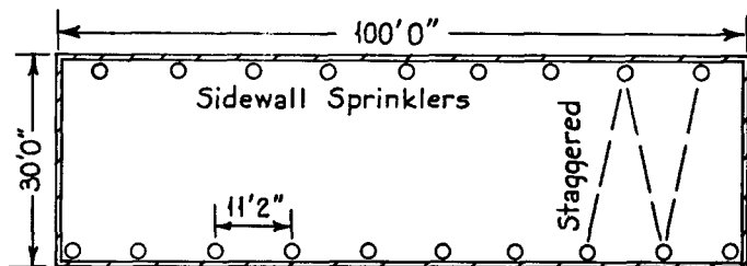
Fig. 4411. Spacing of Sidewall Sprinklers under Smooth Ceilings, with Light Hazard Occupancy.
