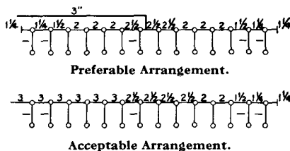
Fig. 3064(a). Arrangement of Two-Sprinkler Branch Lines, Ordinary Hazard Occupancy.
