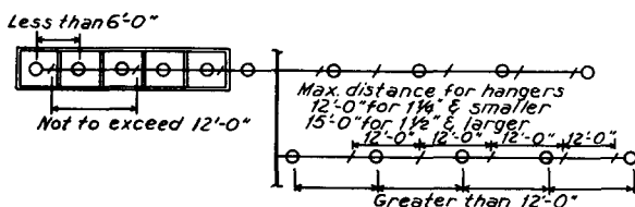
Fig. 3551. Distance Between Hangers.
