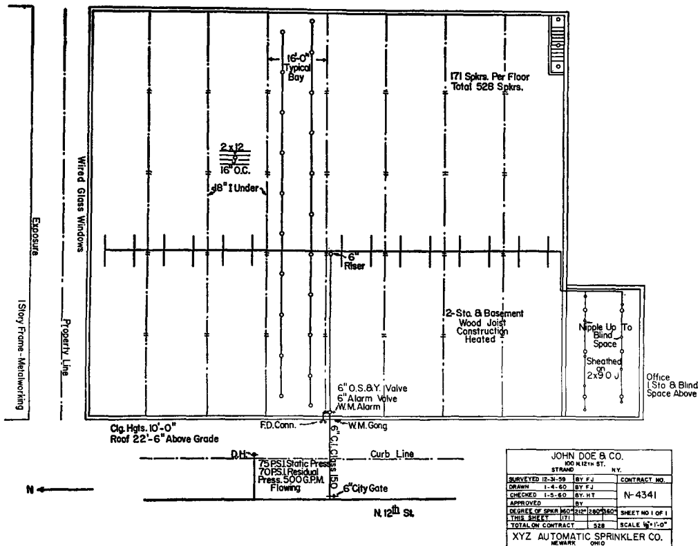
Fig. 1430. Typical Preliminary Plan.
