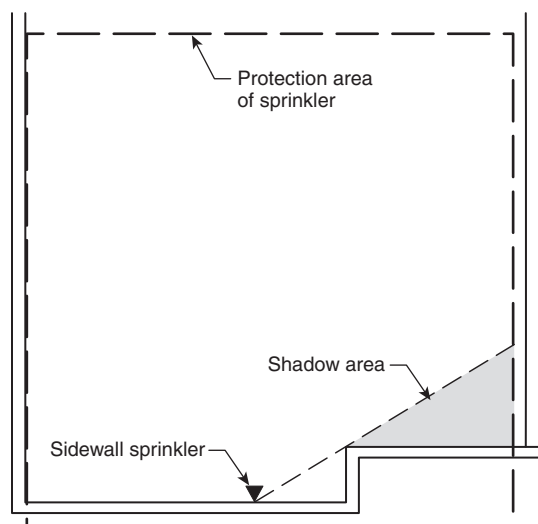
FIGURE A.8.2.5.6(b) Example of Shadow Areas (HSW).
