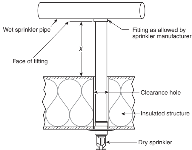
▲ FIGURE A.8.2.6(a) Dry Sidewall Sprinkler Through Wall.
