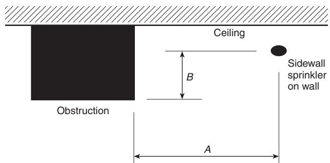
Elevation View
