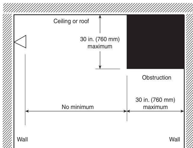
Elevation View
