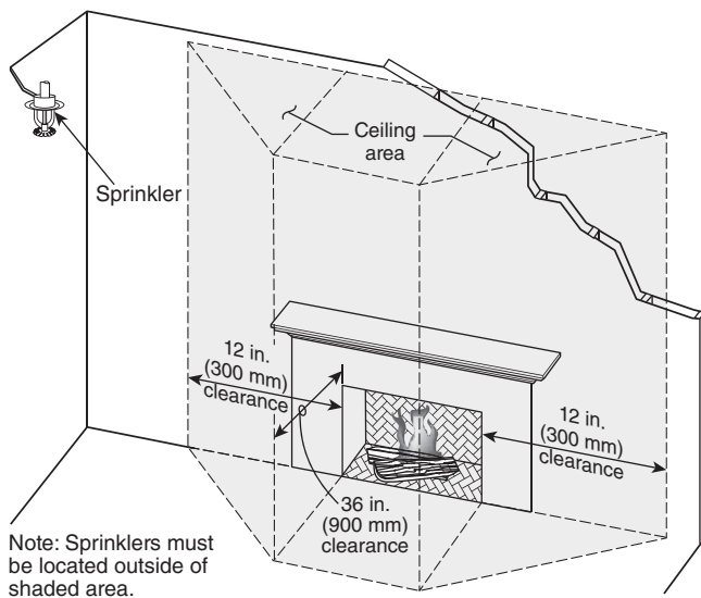
Δ FIGURE A.7.5.6.3(3)(b) Recessed Fireplace — Intermediate Temperature Sprinkler Location.
