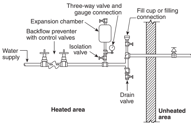
FIGURE 9.2.3.2.1 Arrangement of Supply Piping with Backflow Device.
