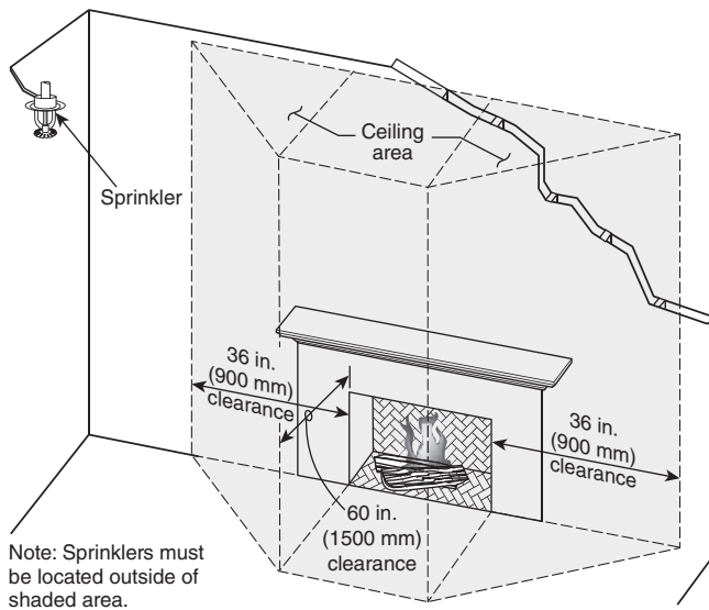
Δ FIGURE A.7.5.6.3(3)(a) Recessed Fireplace — Ordinary Temperature Sprinkler Location.
