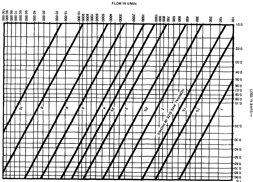
Fig. A-7-2(b) Metric. Friction Loss in Schedule 40 Steel Pipe, Hazen & Williams C-120.
