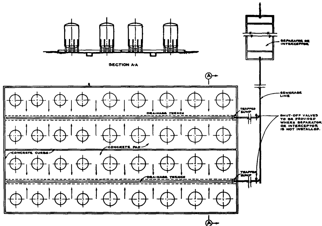
Fig. A-4-6.2(c) Suggested Design for Drainage System for Tank Areas Containing Flammable Liquids.
