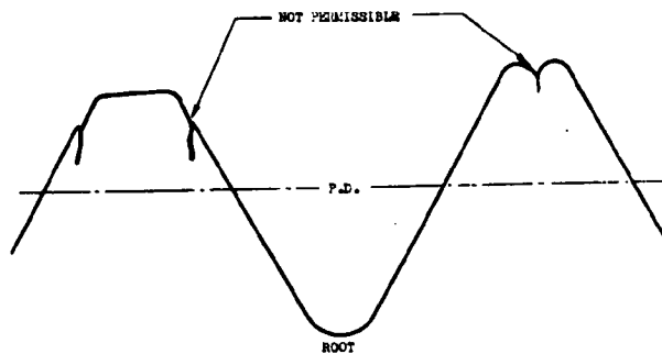
FIGURE 5 ROLLED THREAD
