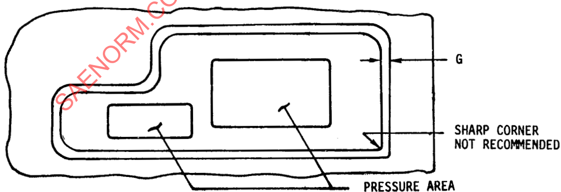
FIGURE 1D EXAMPLE OF NON-CIRCULAR GROOVE CONFIGURATION
