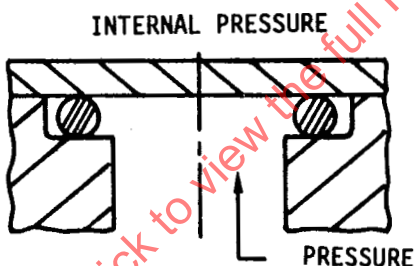
FIGURE 1D EXAMPLE OF NON-CIRCULAR GROOVE CONFIGURATION
