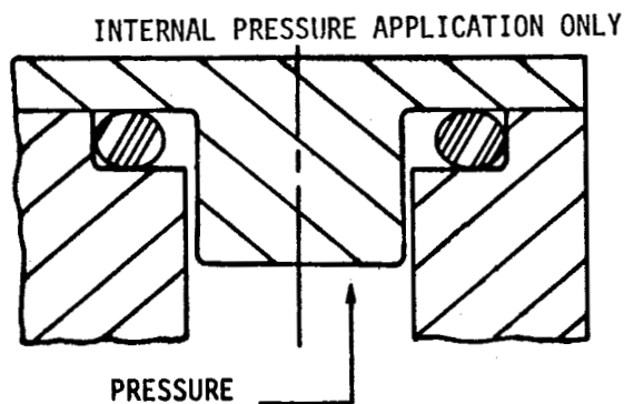
FIGURE 1B O-RING SEAL AXIAL GLANDS ALTERNATE DESIGN
