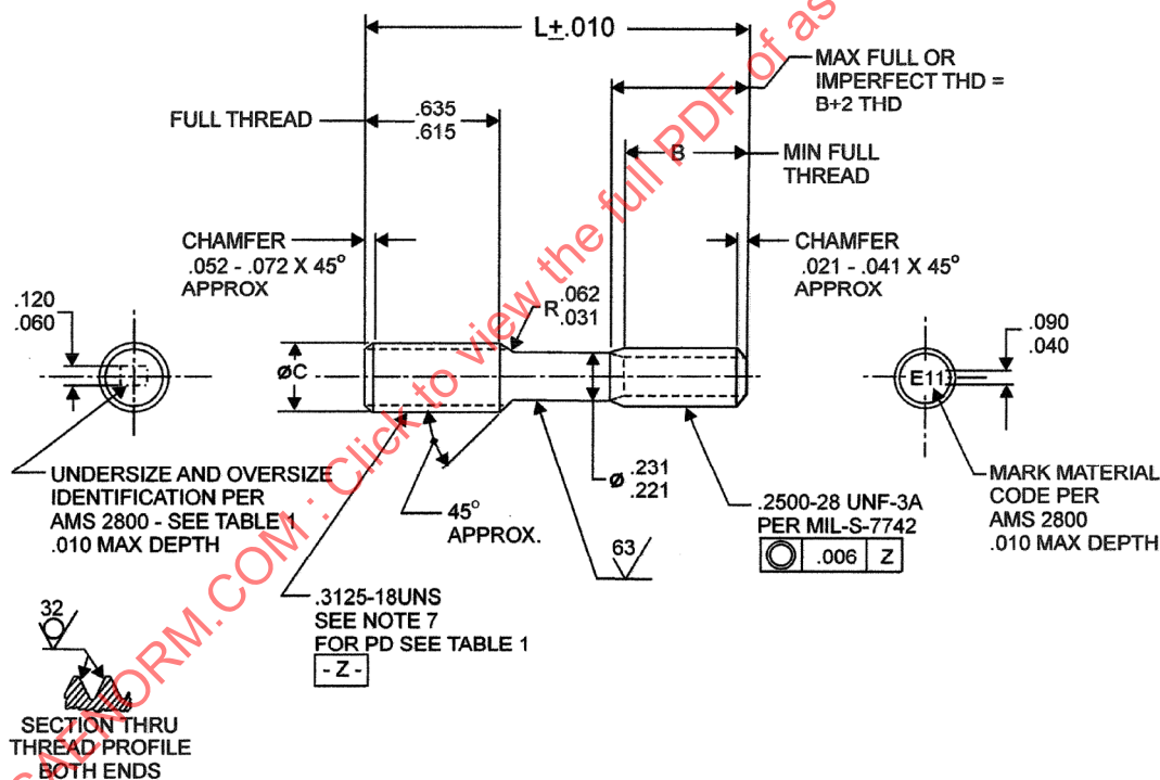
FIGURE 1 - STUD
