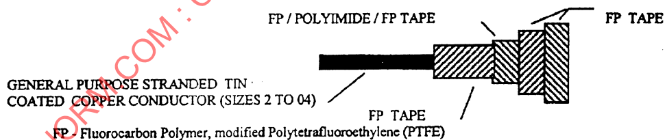
FIGURE 2. GENERAL CONFIGURATION
