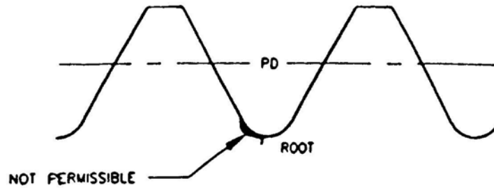
FIGURE 4 - Root Defects, Rolled Thread
