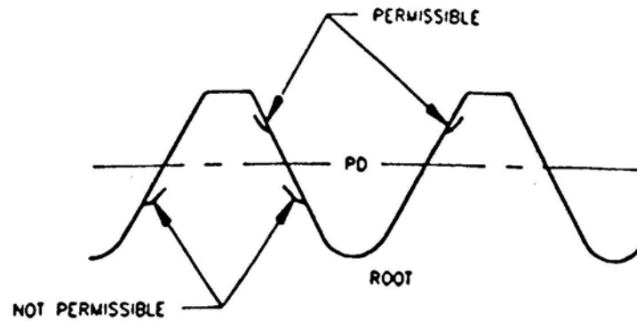
FIGURE 7 - Laps Extending Toward Crest, Rolled Thread
