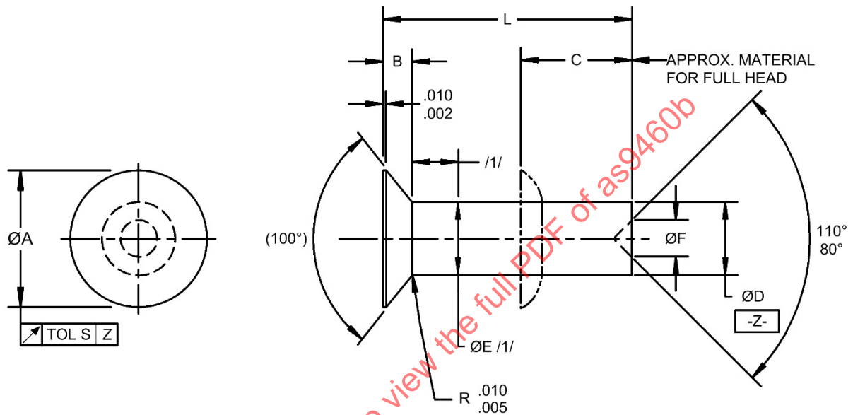
FIGURE 1 - RIVET
