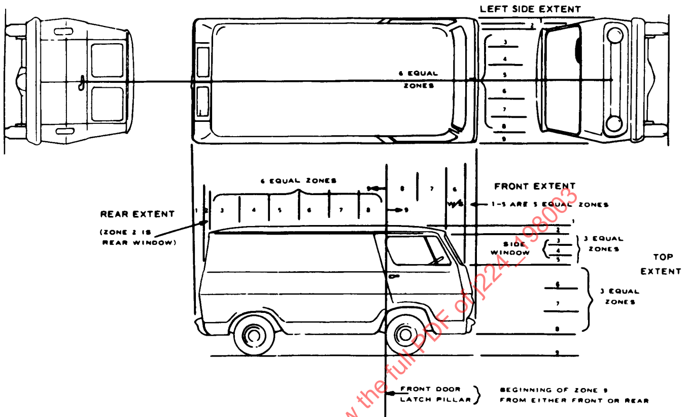
FIGURE 8—DEFORMATION EXTENT ZONES (FOR VANS)
