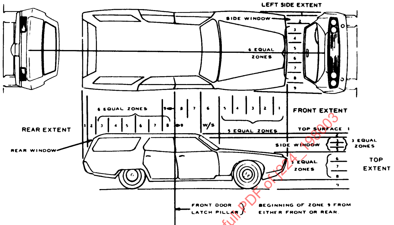
FIGURE 7—DEFORMATION EXTENT ZONES (FOR STATION WAGONS)
