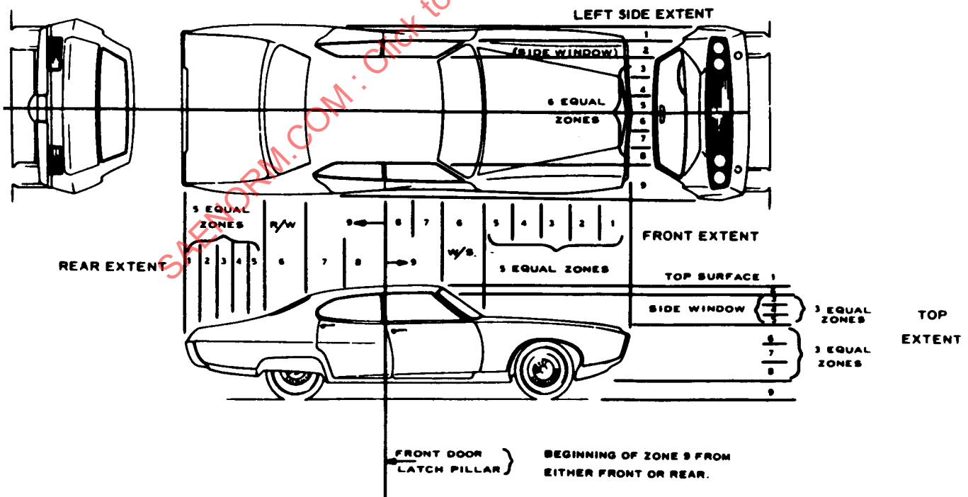
FIGURE 6—DEFORMATION EXTENT ZONES (FOR PASSENGER CARS)
