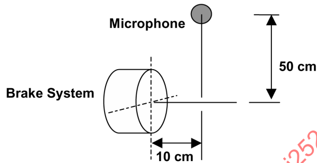
FIGURE 1—MICROPHONE ORIENTATION
