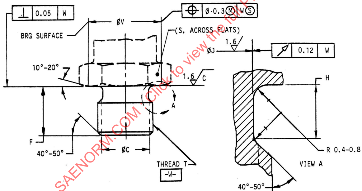
FIGURE 1 - Fitting End Configuration
